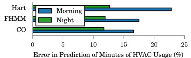
Figure 12: NILM algorithm have high accuracy overall, but have higher error in the morning because other appliances are being used. However, the morning hours are critical to inferring whether a home has a setback schedule.
