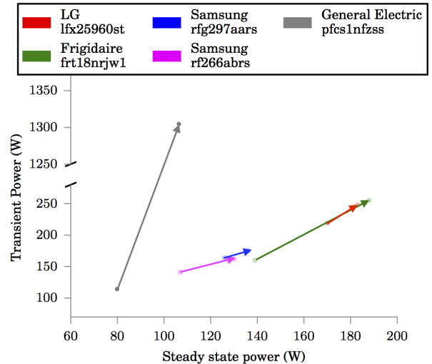
Figure 6: Identical fridges with the same model and age can have differences of 10% or more in steady state power levels. Feedback about failing or mis-configured fridges can save up to 26% energy.
