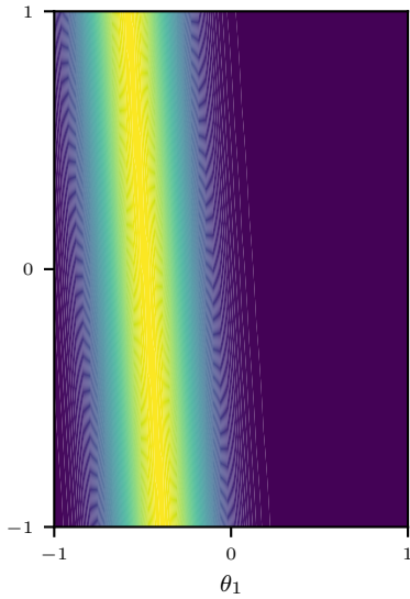
likelihood
