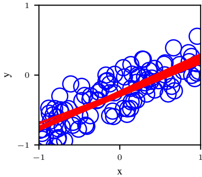
data space
