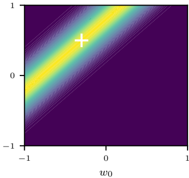
likelihood
